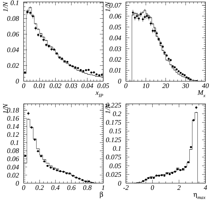
Figure 5.9: The diffractive variables M_X , x_{IP} , \beta and \eta_{max} after altering the \mathcal{R} contribution for the DIFFMY selection.
