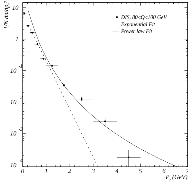
Figure 9.1: The transverse momentum spectra, \frac{1}{N} \frac{dn_{tracks}^{\pm}}{dp_t^2} , as a function of p_t for charged hadrons in the current hemisphere of the Breit frame (statistical errors only). The fits shown are made within restricted p_t ranges but plotted over the whole p_t range.
