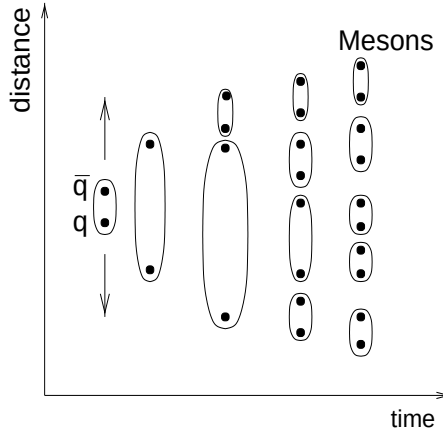
Figure 4.3: The Lund String Hadronisation Model
