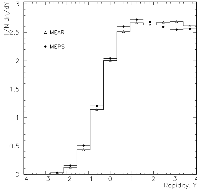
Figure 5.13: The rapidity spectra produced by two different fragmentation models (MEAR and MEPS).
