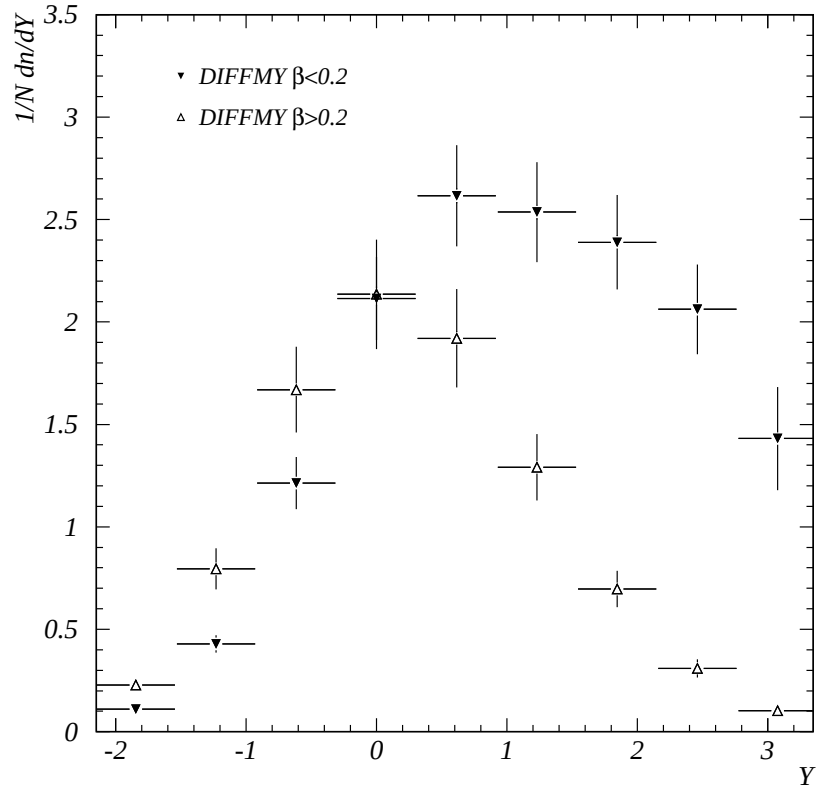
Figure 7.9: Rapidity plateau data comparing DIFFMY for \beta < 0.2 and \beta > 0.2 (statistical and systematic errors).
