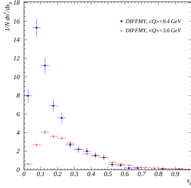
Figure 8.1: The fragmentation function, 1/N dn^{\pm}/dx_p , of the DIFFMY event selection for the current hemisphere of the Breit frame (raw distributions and statistical errors only).
