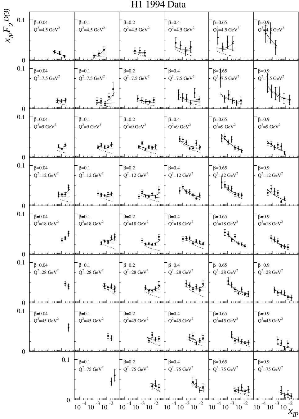
Figure 3.2: The diffractive structure function F_2^{D(3)} . The curves show Regge fits, the dashed curve is the contribution from the pomeron only, the dotted curve shows pomeron + interference, the solid curve shows the total pomeron + interference + reggeon contributions.
