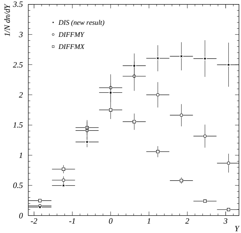
Figure 7.8: Rapidity plateau data comparing DIS, DIFFMX and DIFFMY selections (statistical and systematic errors).
