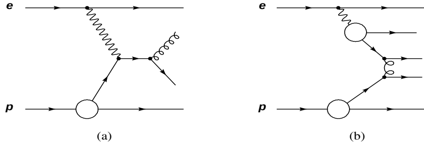
Figure 2.5: (a) Direct and (b) resolved Photoproduction processes.
