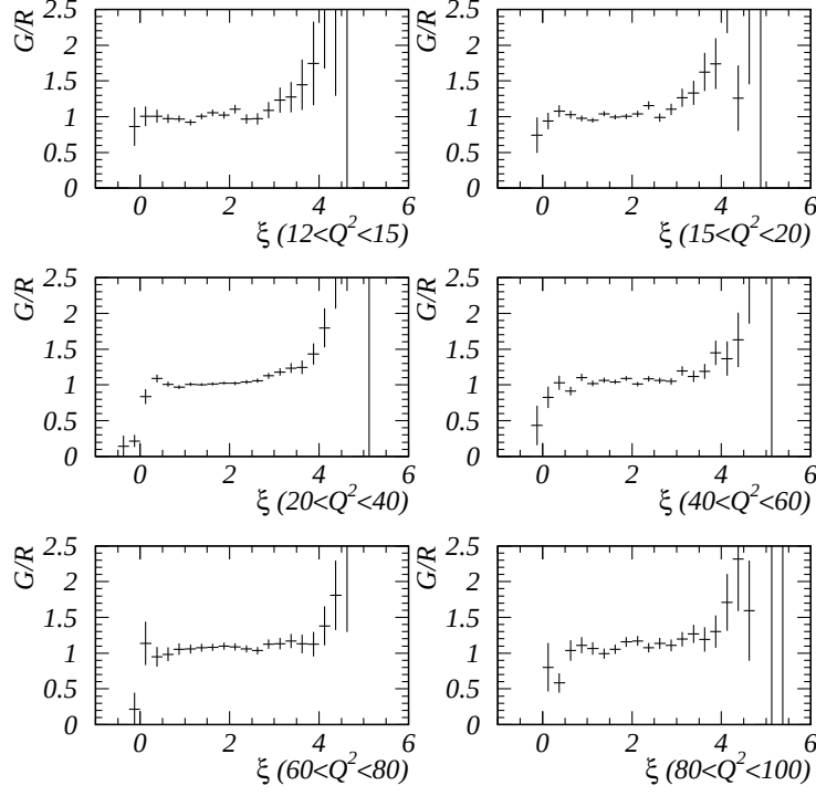
Figure 8.4: Acceptance correction factors applied to the data for the DIFFMY event selection (statistical errors only).
