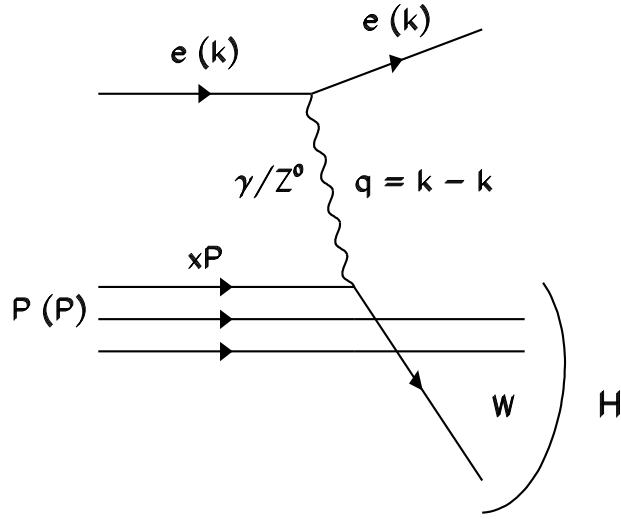
Figure 2.1: Deep Inelastic scattering
