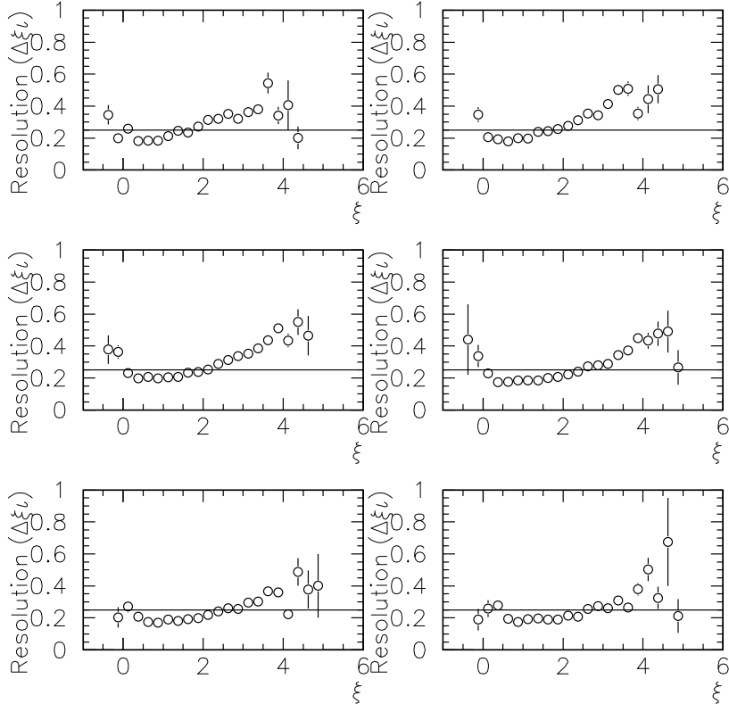
Figure 8.5: The resolution in \xi as a function of \xi for the DIFFMY event selection. The solid line shows the bin-width ( \xi \sim 0.25 ) (statistical errors only).
