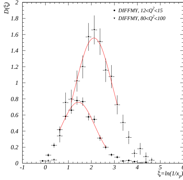
Figure 8.14: The fragmentation function, D(\xi) , for the DIFFMY event selection after acceptance corrections together with Gaussian fits in the region of the peak. (corrected distributions and statistical errors only)
