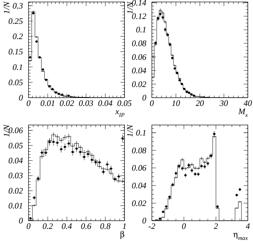
Figure 5.11: The diffractive variables M_X , x_{\mathbb{P}} , \beta and \eta_{max} for the DIFFMX event selection.
