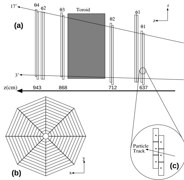
Figure 1.9: The Forward Muon Detector (FMD)
