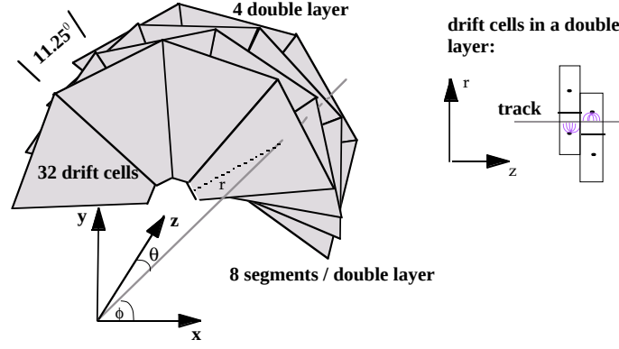
Figure 1.4: Schematic view showing the rotated layers and sectors of the BDC.
